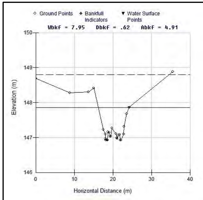
Figure 16: Cross Section D2
