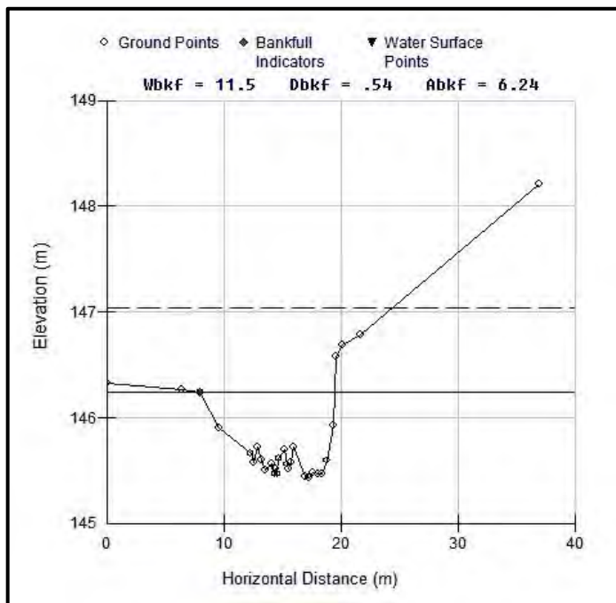
Figure 18: Cross Section D4
