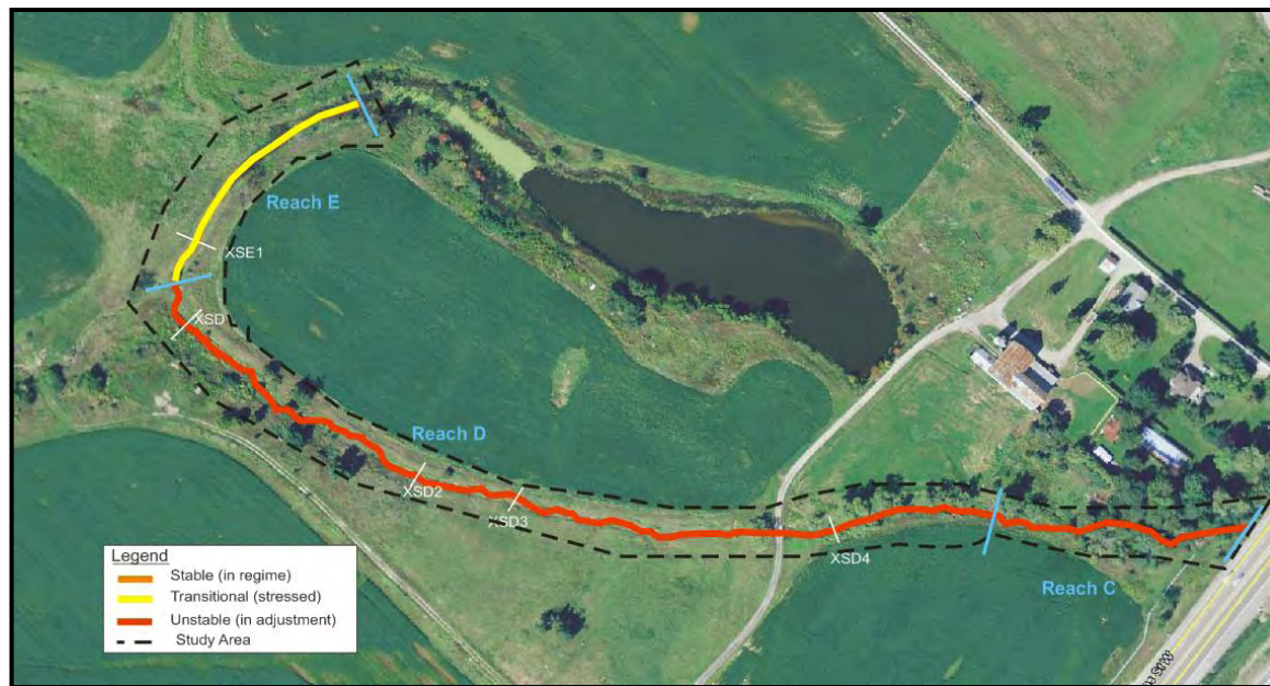
Figure 5: RGA Results for Reaches C, D and E
