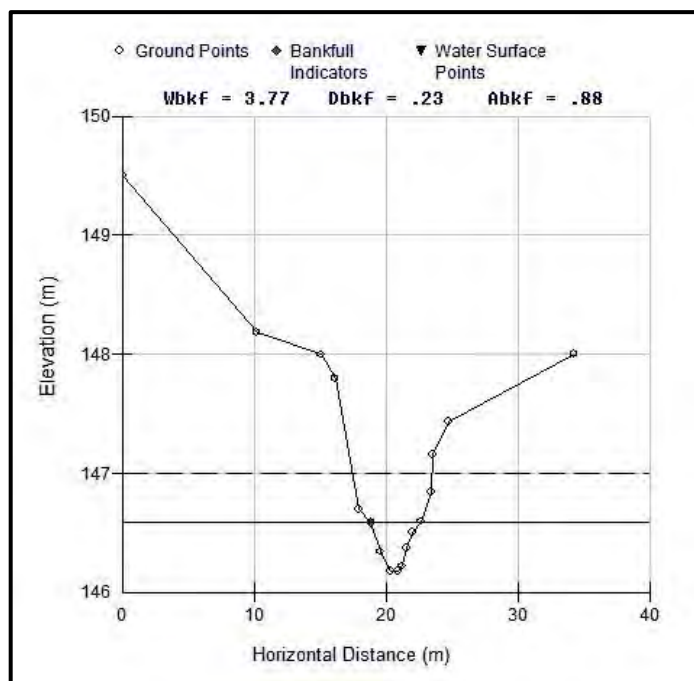
Figure 17: Cross Section D3
