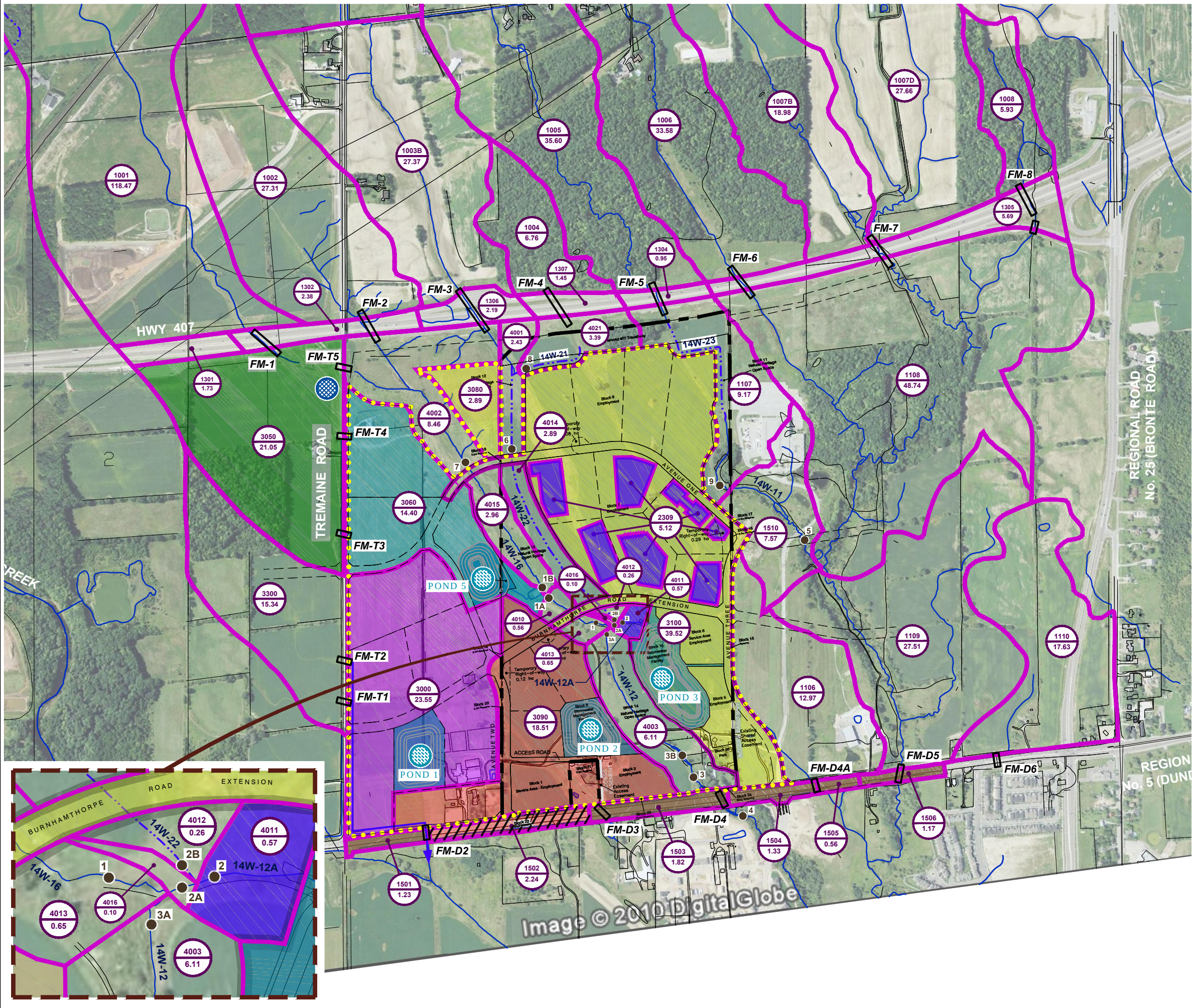
FIGURE 7.4.5.dwg - Ultimate Drainage Boundaries & Reference Nodes 1:11441 Projects by Job Number/2017/09222-001-Lazy Pat Farm Property June 2017/Figures/ Jun 02, 2017 - 4:29pm
